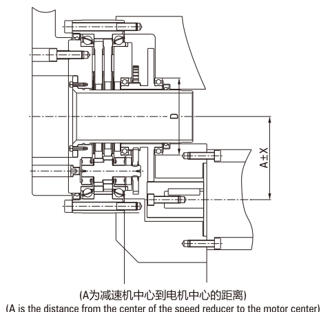
● 图 D.1: RVC系列装配精度 Figure D.1: RVC series assembly precision
